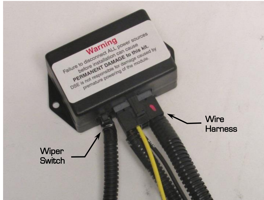
Figure 25– Connect Wiper Switch & Harness to Module
