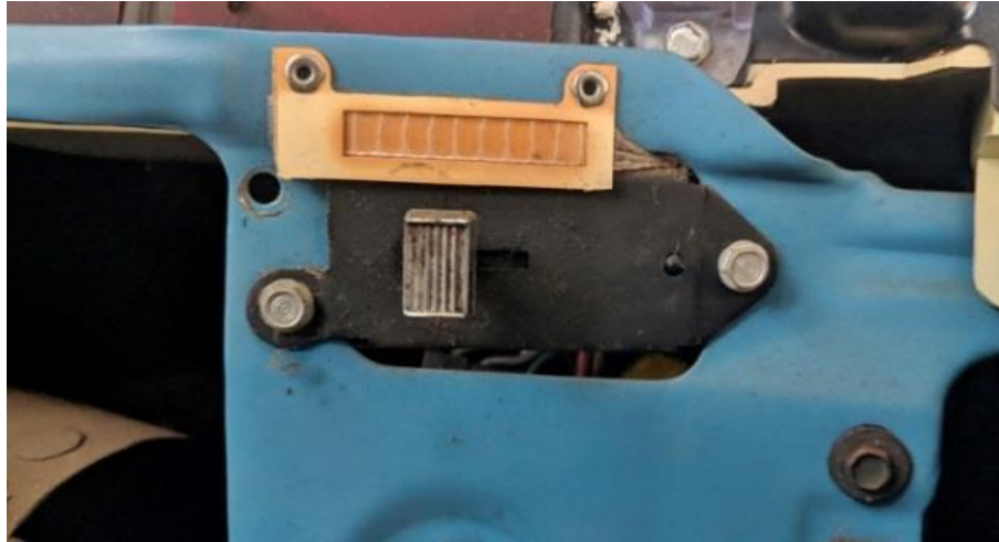
Figure 5 – Remove Factory Wiper Switch (1973-74 shown)
