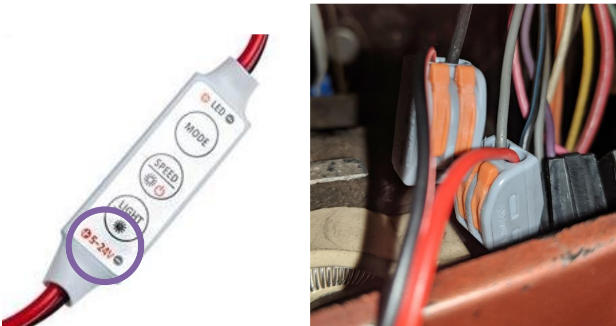
Figure 11 - Connect 5-24V side of LED Dimmer to Original Light Bulb Wires
