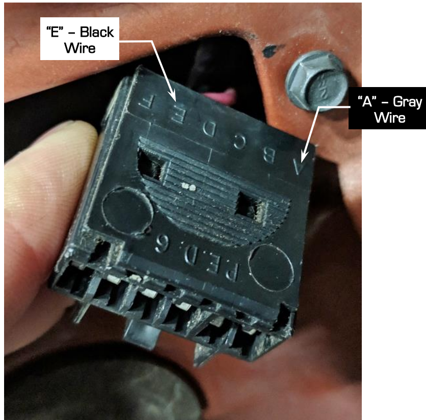
Figure 6 – Cut “A” & “E” Wires
