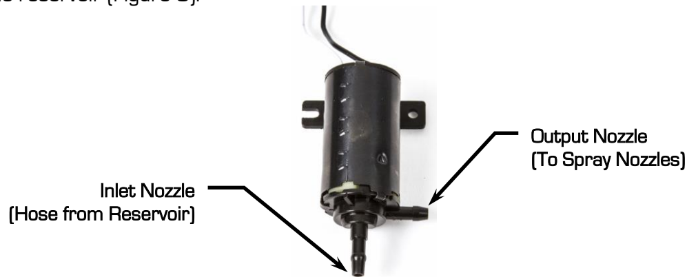
Figure 3 - Connect Hoses to Washer Pump
