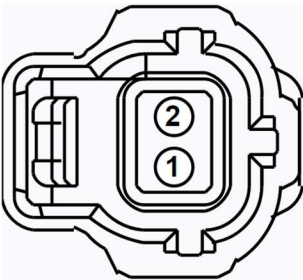
C1B: Inline from Main to Transmission Harness
