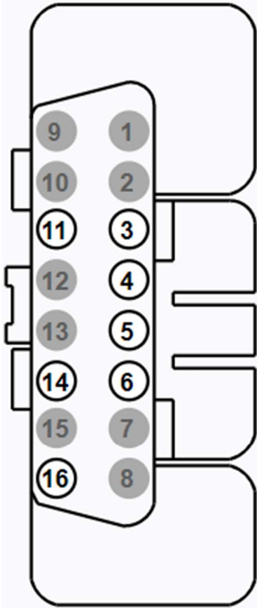
C102A: Alternator
